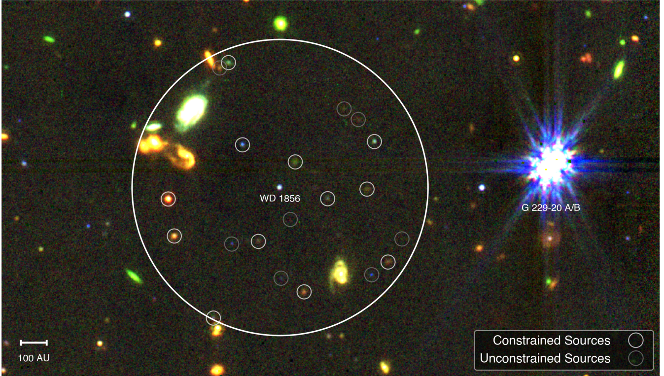
Figure 1. False-color image of the WD 1856 system made using three JWST MIRI filters: F770W, F1500W, and F1800W. We label both WD 1856 and its companion M dwarf binary, G 229-20 A/B. We denote WD 1856’s Hill sphere ( R_{\text{HS}} = 570^{+250}_{-170} au, Vanderburg et al. 2020 ; Limbach et al. 2025 ) with a large white circle. To search for additional planets in the system, we measure the proper motions of all sources within this region. Sources with well-constrained motions ( \sigma < 0.5 pixels) are marked in white, and sources with poorly constrained motions are marked in gray. We describe the process of identifying nearby sources and measuring their proper motions in §3.2.
