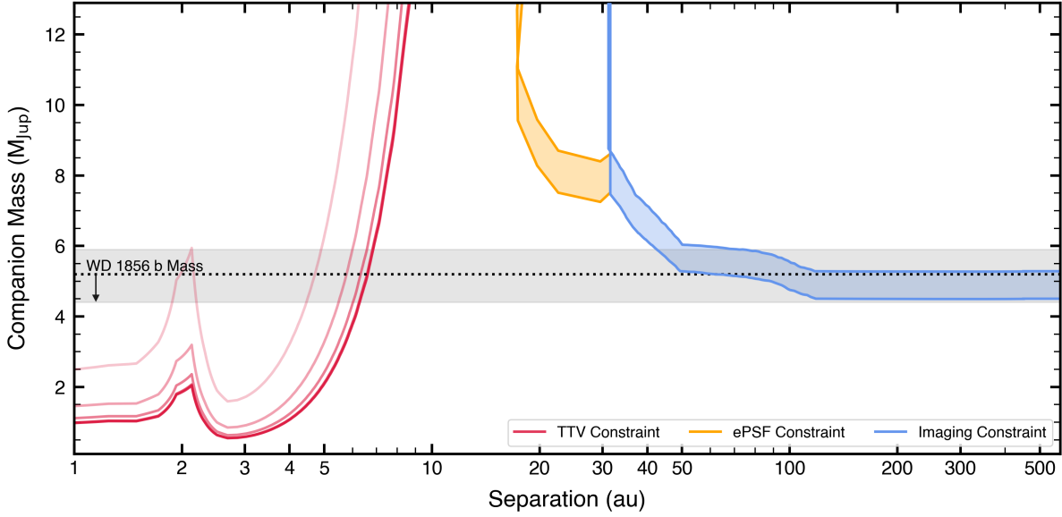
Figure 7. Combined constraints from TTVs and MIRI imaging. We include TTV constraints for companions at a range of inclinations (20, 40, 60, 80, and 90 degrees, with larger values denoted by increasing opacity), and imaging constraints for the system’s expected age range (7.4–10 Gyr). We rule out planets \geq 1 M_{\text{Jup}} at close-in separations and planets \geq 5 M_{\text{Jup}} at wide separations. For comparison, we include an upper limit on the mass of WD 1856 b, with uncertainties denoted by the gray shaded region. Any less massive perturbing companion would likely have been ejected from the system.
