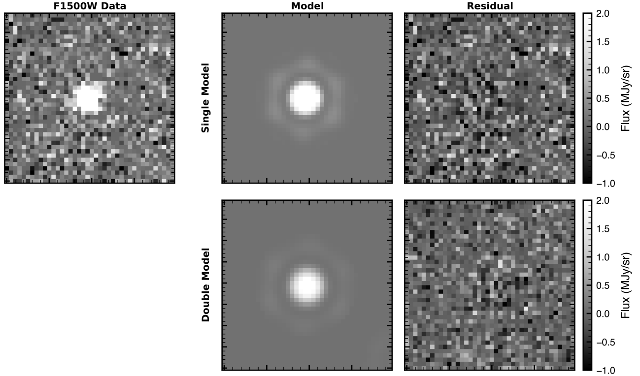
Figure 3. Empirical PSF fits. To search for close-in companions, we simultaneously fit WD 1856 in the four F1500W dithers from both visits. Here we show the data, best-fit models, and residuals for the first dither. We find that the double PSF model has a higher BIC and AIC than the single PSF model. Additionally, the Bayes factor B indicates that there is no evidence the double PSF model is preferred. We therefore conclude that there is no detection of a close-in planet.
