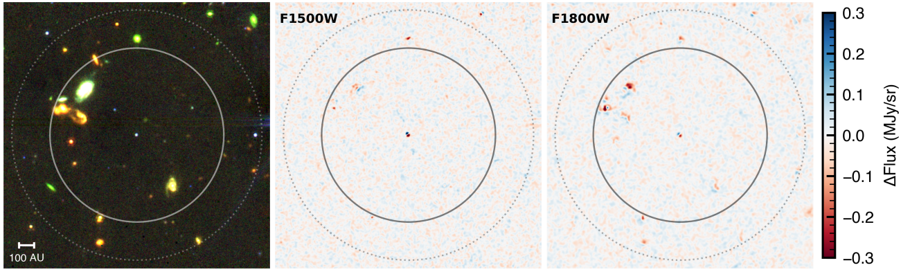
Figure 4. Difference images in both the F1500W and F1800W filters, smoothed with a Gaussian kernel matching the instrument PSF. Distant background objects show negligible apparent motion, and therefore have small residuals. In contrast, nearby and fast-moving objects produce prominent positive and negative residuals. The white dwarf, center, exhibits clear motion. No other sources appear to be co-moving with the white dwarf. The Hill sphere radius is denoted by white and black circles in each image, while its corresponding 1\sigma upper limit is denoted by white and black dotted lines. Left: False-color image. Middle: Difference image in the F1500W filter. Right: Difference image in the F1800W filter.
