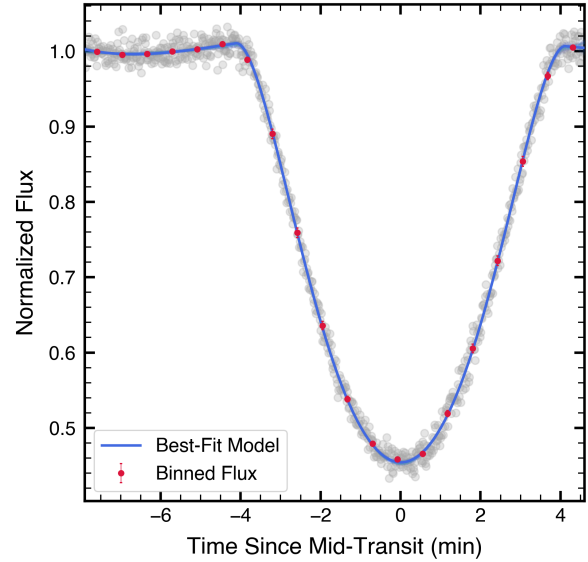
Figure 2. Photometric data from qCMOS photometry. Binned data is shown in red and the best-fit model is shown in blue. We use the best-fit transit time to provide updated TTV constraints on the presence of any existing outer companions.
