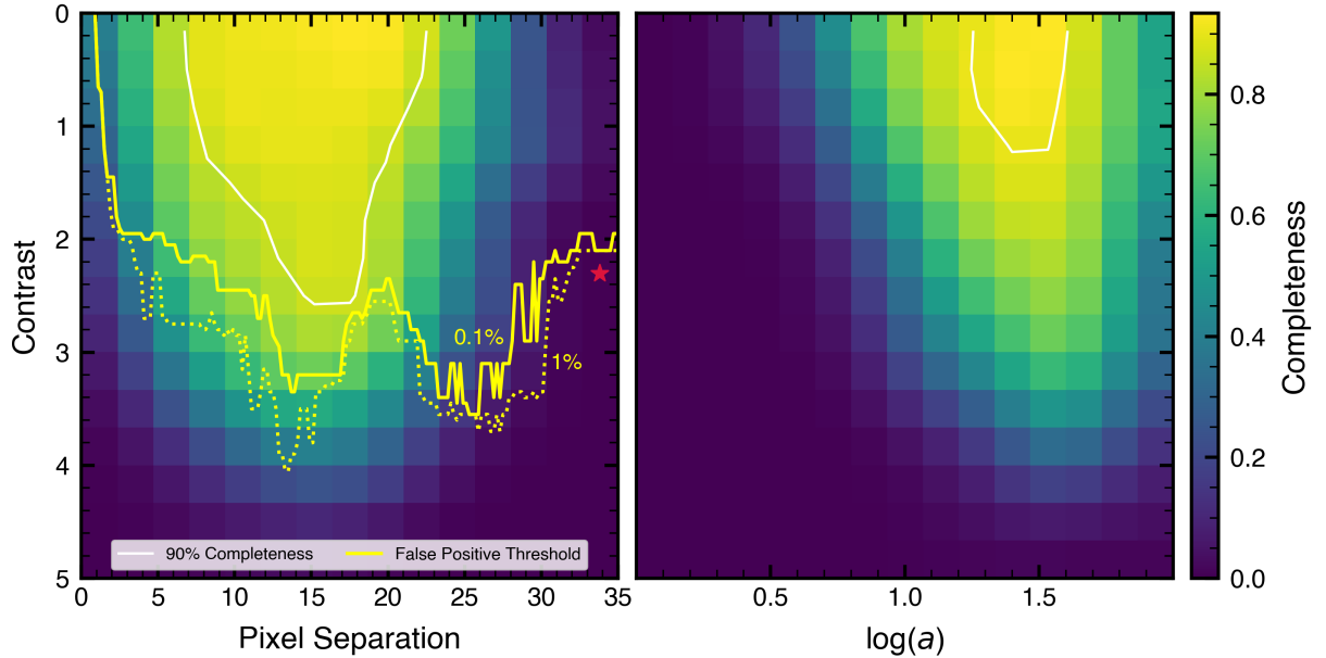
Figure 6. Completeness in the F1500W filter as a function of pixel separation (left) and semimajor axis (right). We randomly generate 20,000 synthetic planets with a range of contrasts and separations, as described in §4.1. We show both the 90% recovery threshold and the 0.1% false positive curve in white and yellow, respectively. We are able to reliably recover companions beyond \sim 5 au, and are primarily sensitive to companions with contrasts < 2.6 mag. The best-fit companion, denoted by the red star, falls well outside the 90% completeness boundary and below the 1% false positive curve, suggesting it is not a real source.
